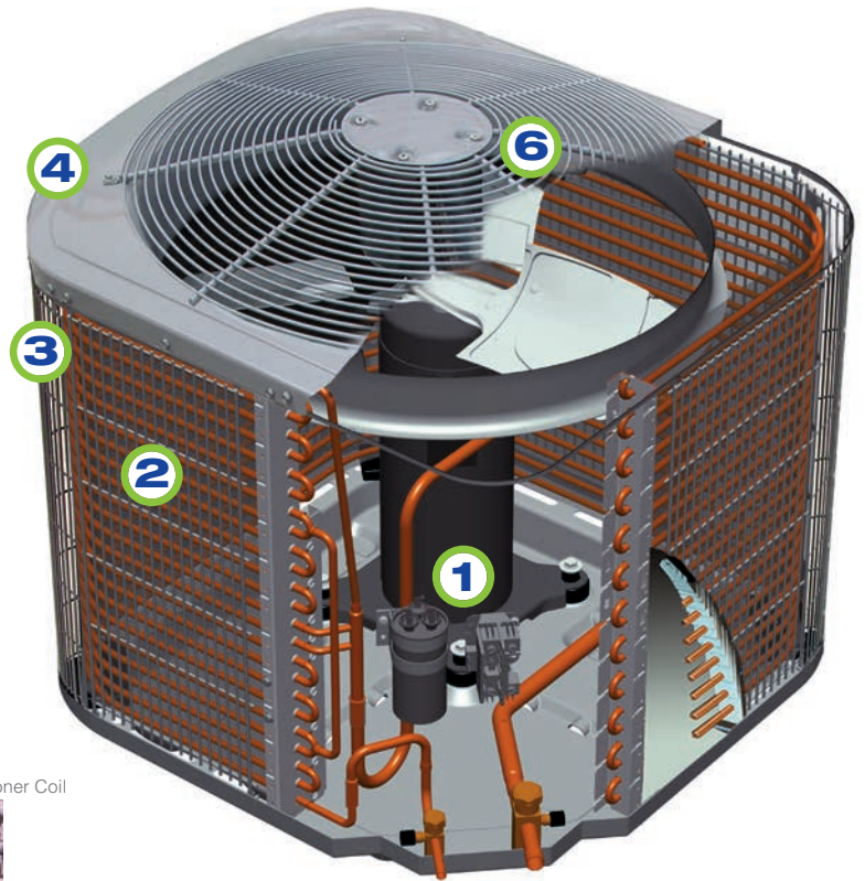
Comfort™ 13 Air Conditioner Coil with ArmorPlate™ Coating
